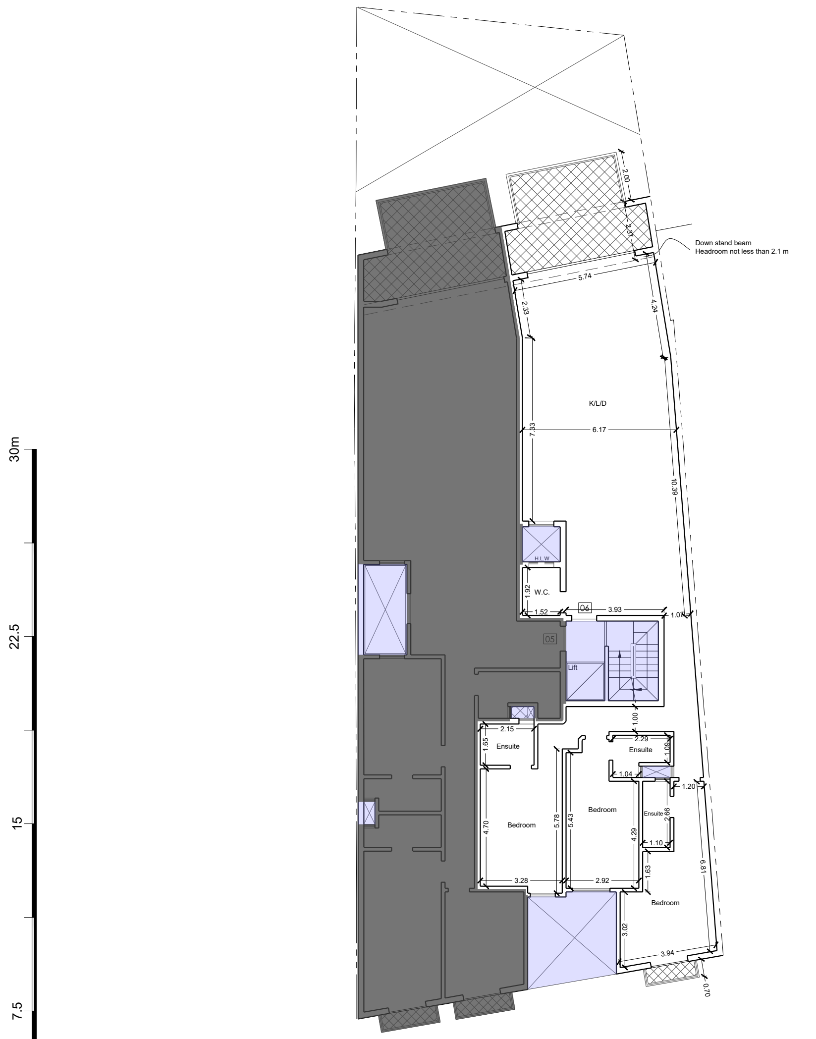
First Floor Level 1
